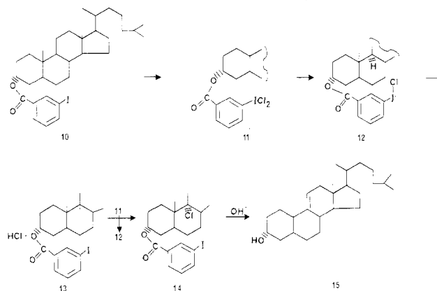
Scheme III Radical-Relay Chlorination Directed by a Template
